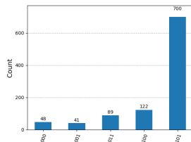
Figure: Addition=2 + 3 operation with QCCircuits and simulator.
