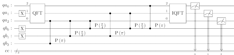
Figure: Partial implementation of AF
